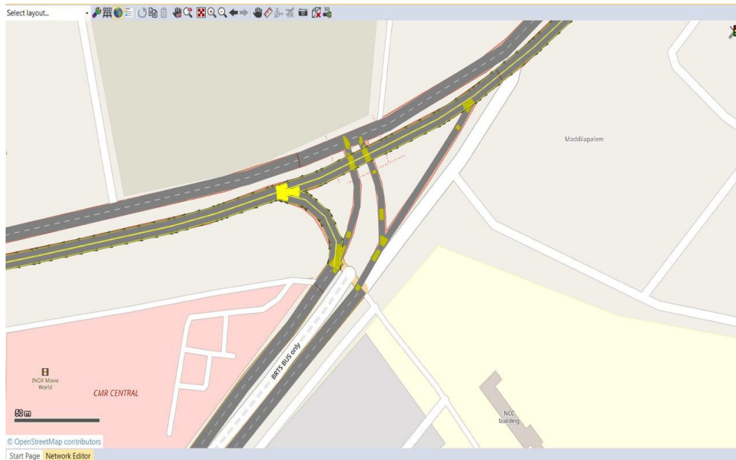
Fig 3: Map from VISSIM Software for Maddilapalem Junction
