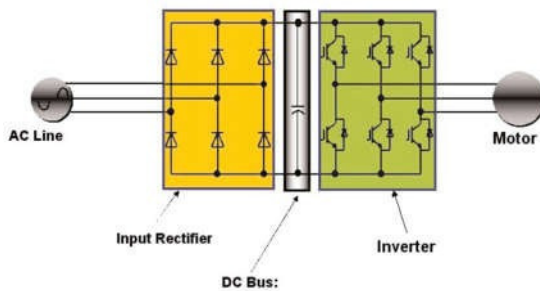
Fig. 3.2. VFD basics: Existing technology
